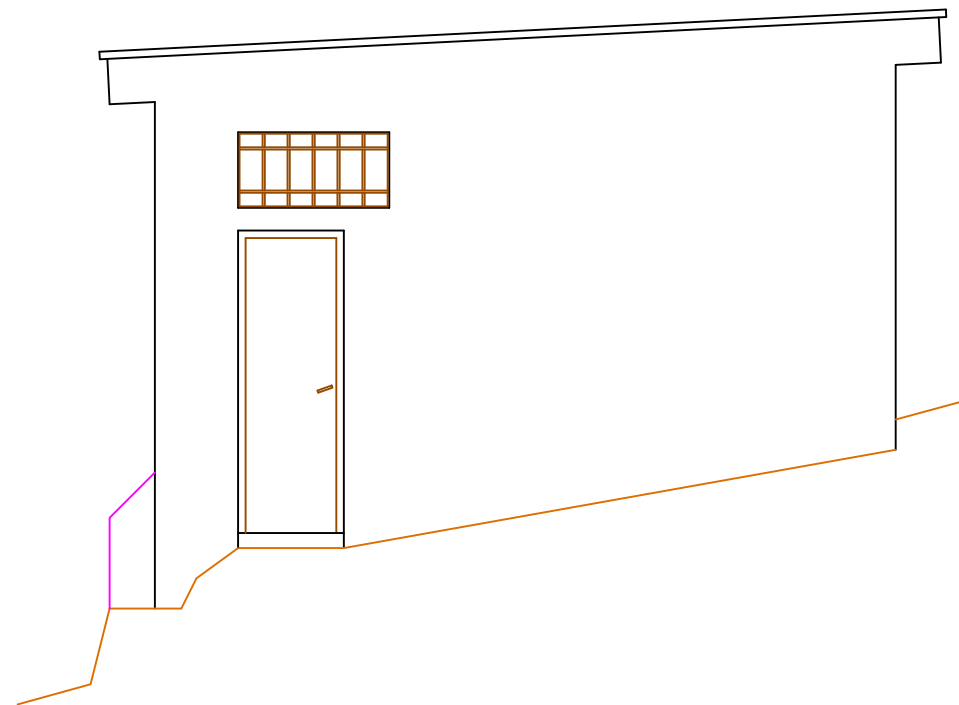
Alzado Principal
